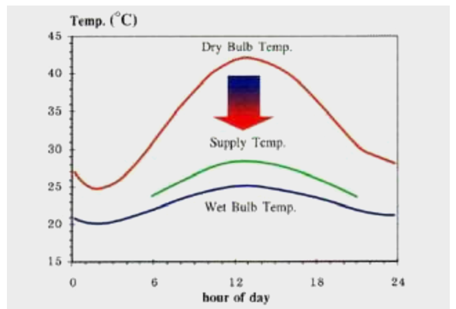
Temperature reduction during the day by CeLPad System (Tropical Area)
